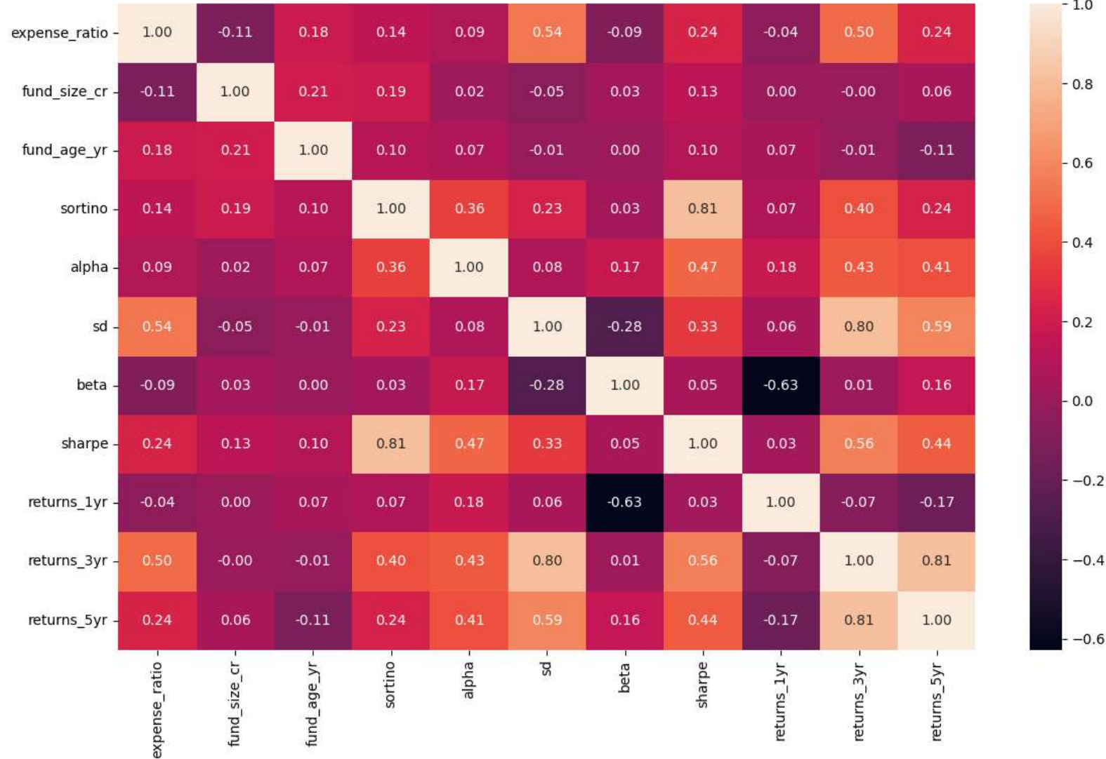
Correlation Matrix
